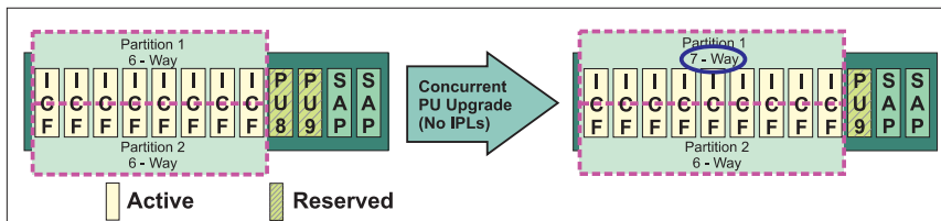
Figure 24. Shared internal coupling facility
