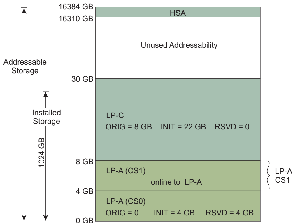
Figure 28. Reconfigured central storage layout
