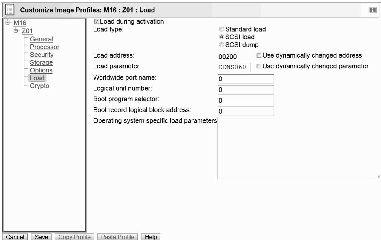
Figure 44. Load page, image profile
