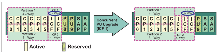
Figure 23. Multiple dedicated PR/SM partitions
