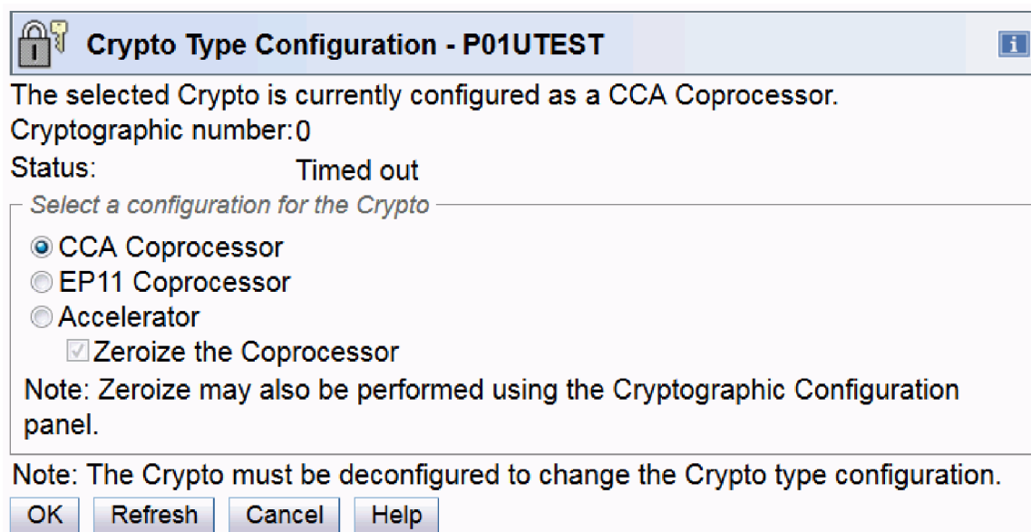
Figure 70. Crypto type configuration window
