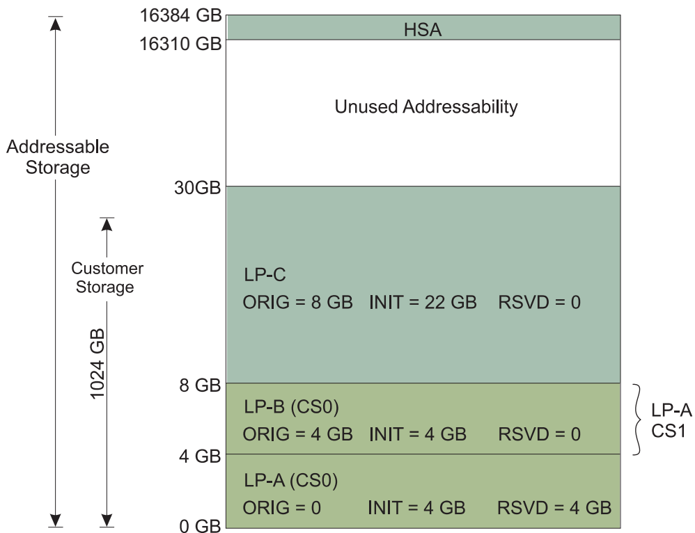
Figure 27. Central storage layout
